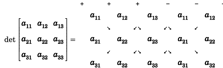
Figure C.1 Evaluating a 3 \times 3 determinant
