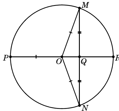
Figure 1 Pieri's 1900 definition of Q lying between P, R
