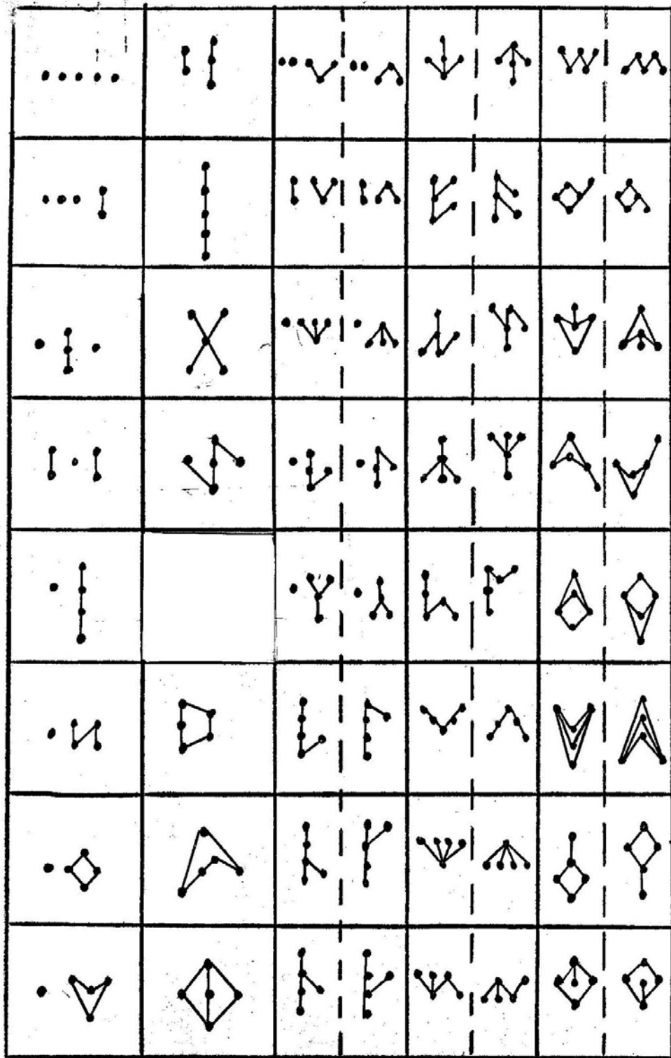
The 63 five-node Hasse diagrams
